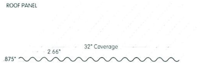
ROOF PANEL
