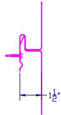
DETAIL B SIDE VIEW
